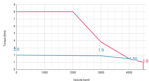
Motor Curve ACTILINK-SC 6-3
