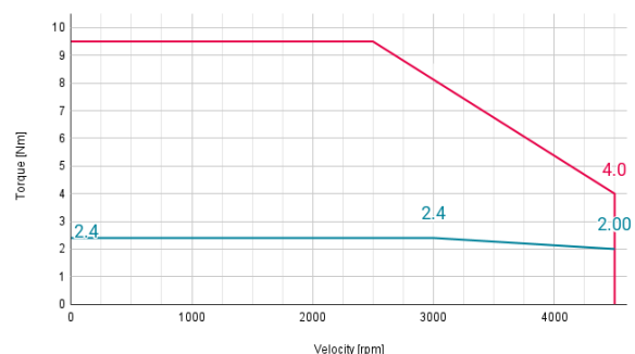
Motor Curve ACTILINK-SC 8-1
